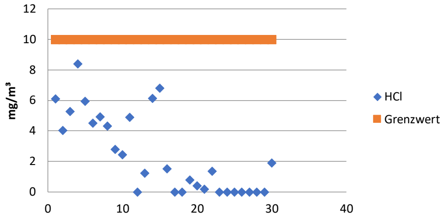
HCl - April 2019
